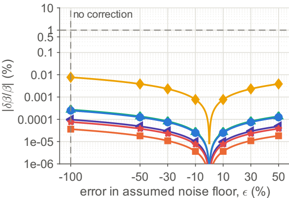
(a) Stiffness error
